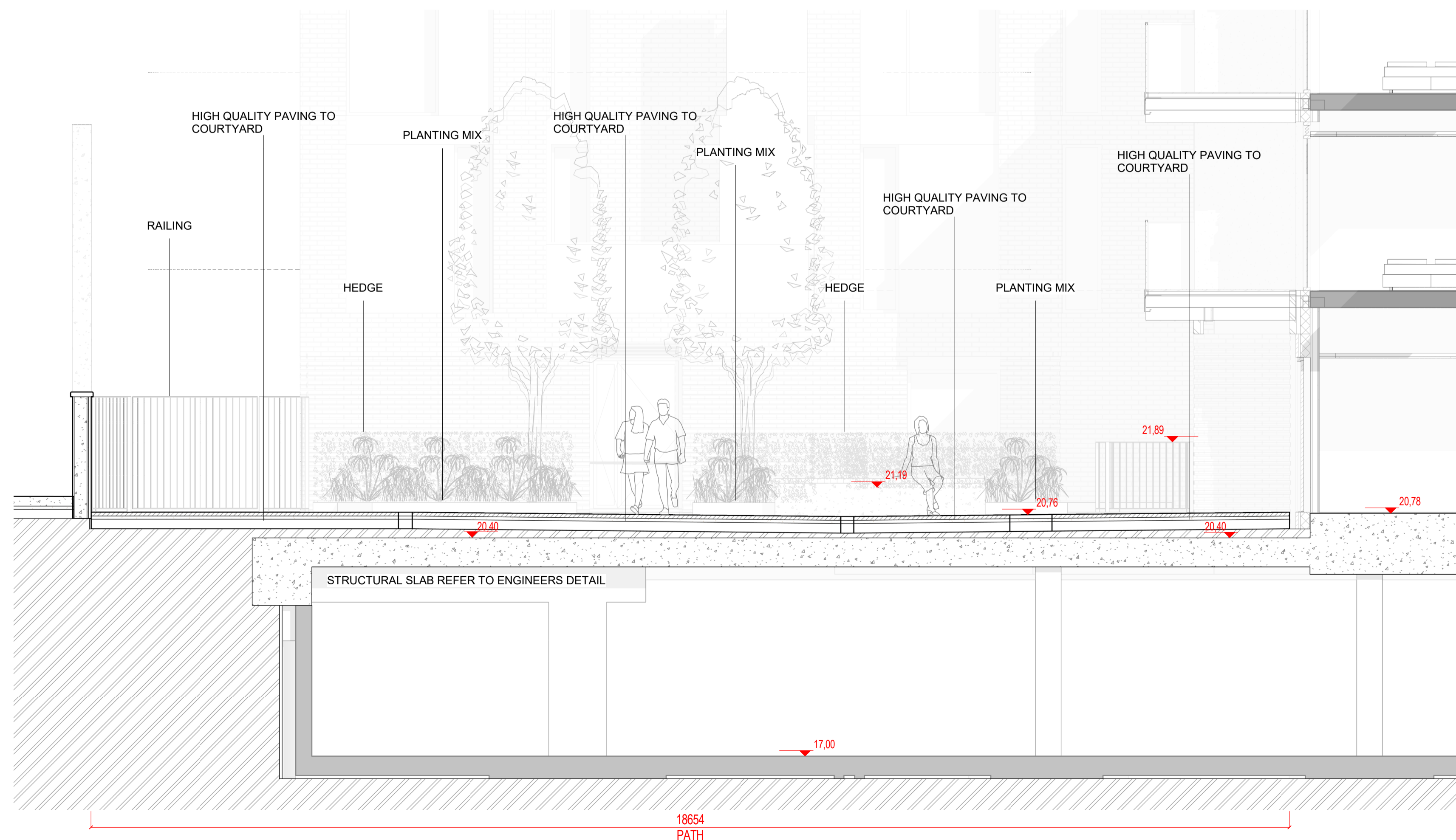
2 COURTYARD SECTION - BG3 4 1:50 @A1
