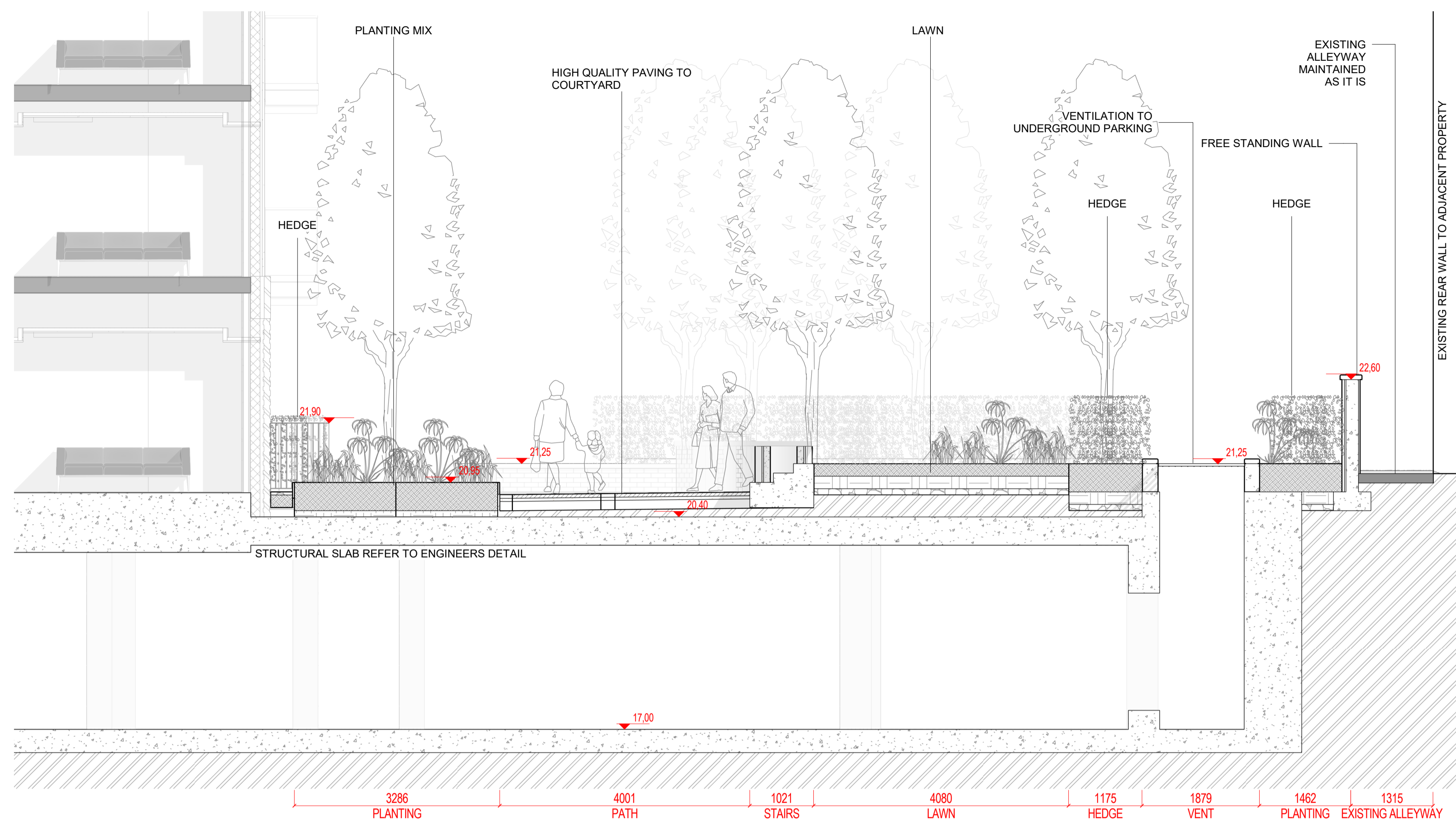
1 COURTYARD SECTION - BG3 3 1:50 @A1
